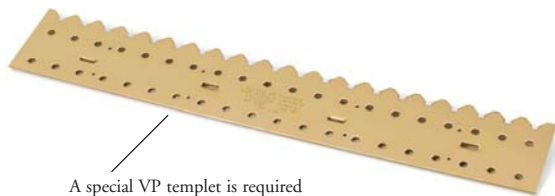
A special VP templet is required for proper bolt-hole spacing. Templet is yellow dichromate plated for easy identification.
