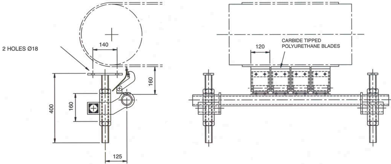
Multiblade Scraper
