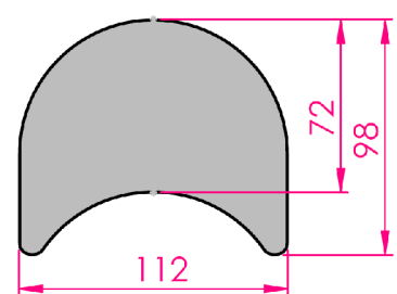
TOP CHAIN DIMENSIONS (NOT TO SCALE)
